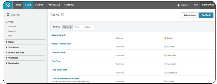
Web-based automation with MOVEit Automation
